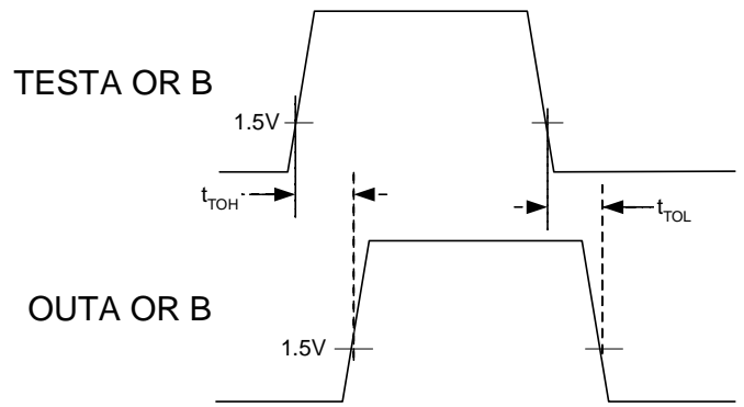
Figure 4 TEST Input to Logic Output Switching Waveform
