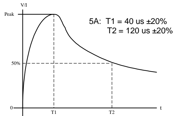
Figure 7 DO160 Lightning Induced Transient Voltage Waveform #5.
