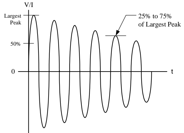
Figure 5 DO160 Lightning Induced Transient Voltage Waveform #3 Pin Injection Voc = 600 V, Isc = 24 A. Freq = 1 MHz ±20%
