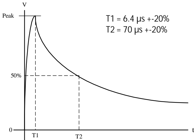
Figure 4 DO160 Lightning Induced Transient Voltage Waveform #4 Pin Injection Voc = 300 V, Isc = 60 A
