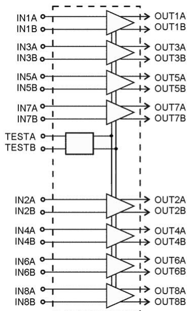
Figure 1 DEI1049 Block Diagram and Truth Table
