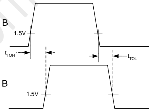
Figure 4 TEST Input to Logic Output Switching Waveform
